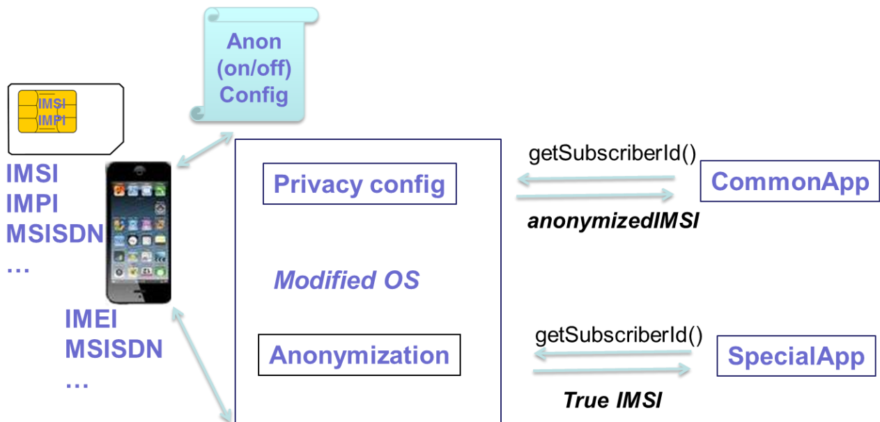
Figure 6 Device-based Anonymization.
